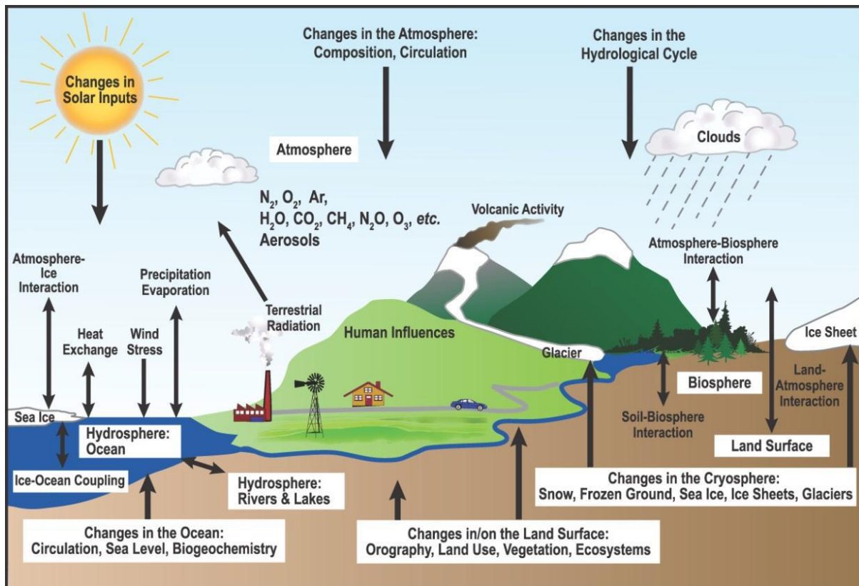
Figure 2.1.6: Schematic view of the components of the climate system, their processes and interactions [IPCC Fourth Assessment Report, Climate Change 2007 (AR4) WG I]
