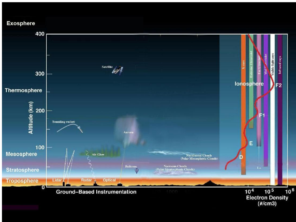
Fig 2.1.5: Diagram of the layers within Earth's atmosphere.
