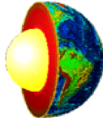
Fig 2.1.1: The Lithosphere
