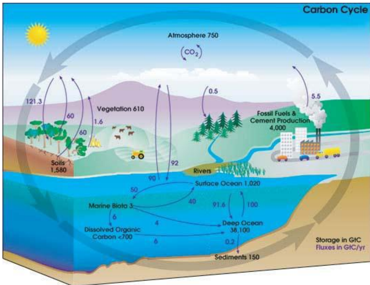
Figure 2.3.1: Major Carbon pools and fluxes of the global carbon balance [FAO website]
