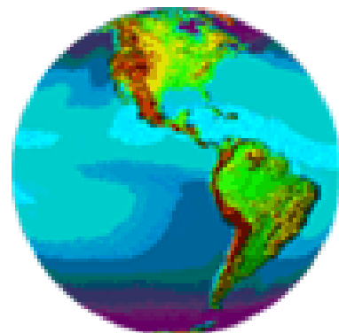
Fig 2.1.2: The Hydrosphere
