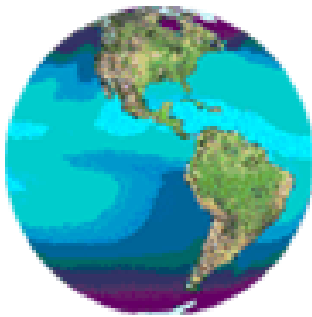
Fig 2.1.3: The Biosphere.
