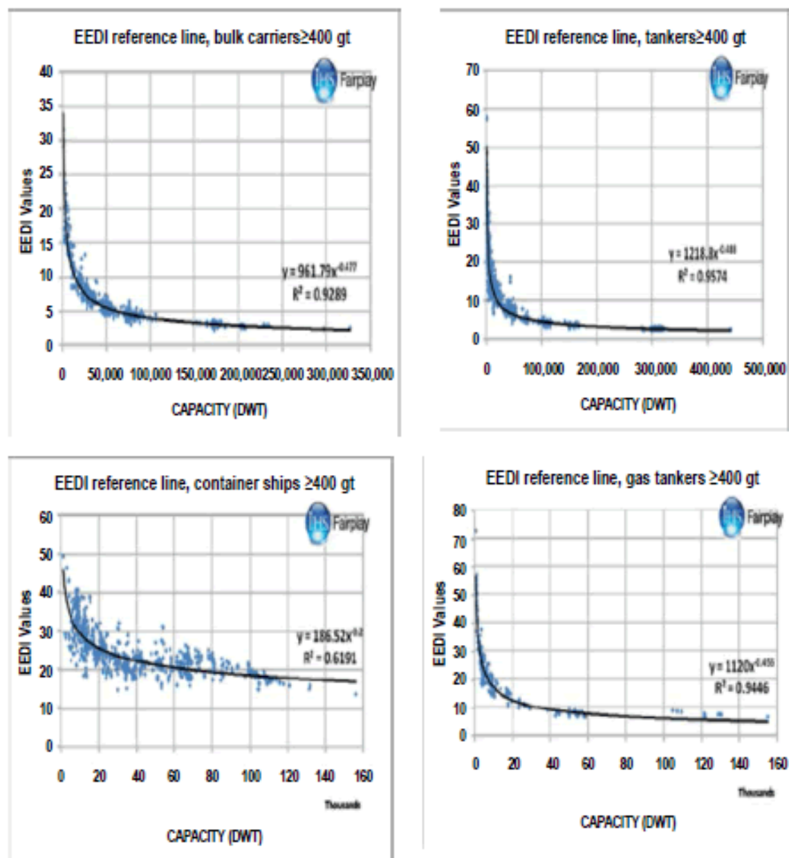
Figure 2: EEDI Reference Lines as developed by the IMO using techniques in Resolution MEPC.231(65)) Note: Reprinted from Module 2 - Ship Energy Efficiency Regulations and Related Guidelines, IMO.
